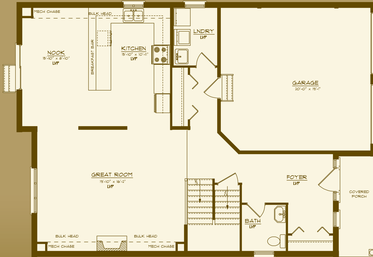
Main Floor 1,121 Sq. Ft.
